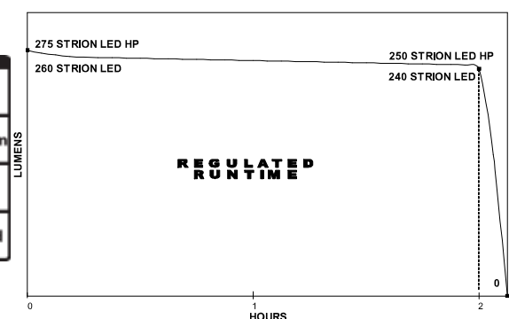
PERFORMANCE CURVE
